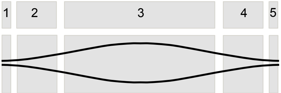
Fig. 3. The regions of an average reed aperture (after moistening). Regions 1 and 5 are the corners; region 3 is the center or primary curve; regions 2 and 4 are the mid-portions, sometimes containing secondary curves (recurves).
