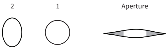
Fig. 7e. When wire 2 is deformed into a vertical oval, the aperture closes, especially in the off-axial portions (shaded), often increasing the secondary curves (recurves).
